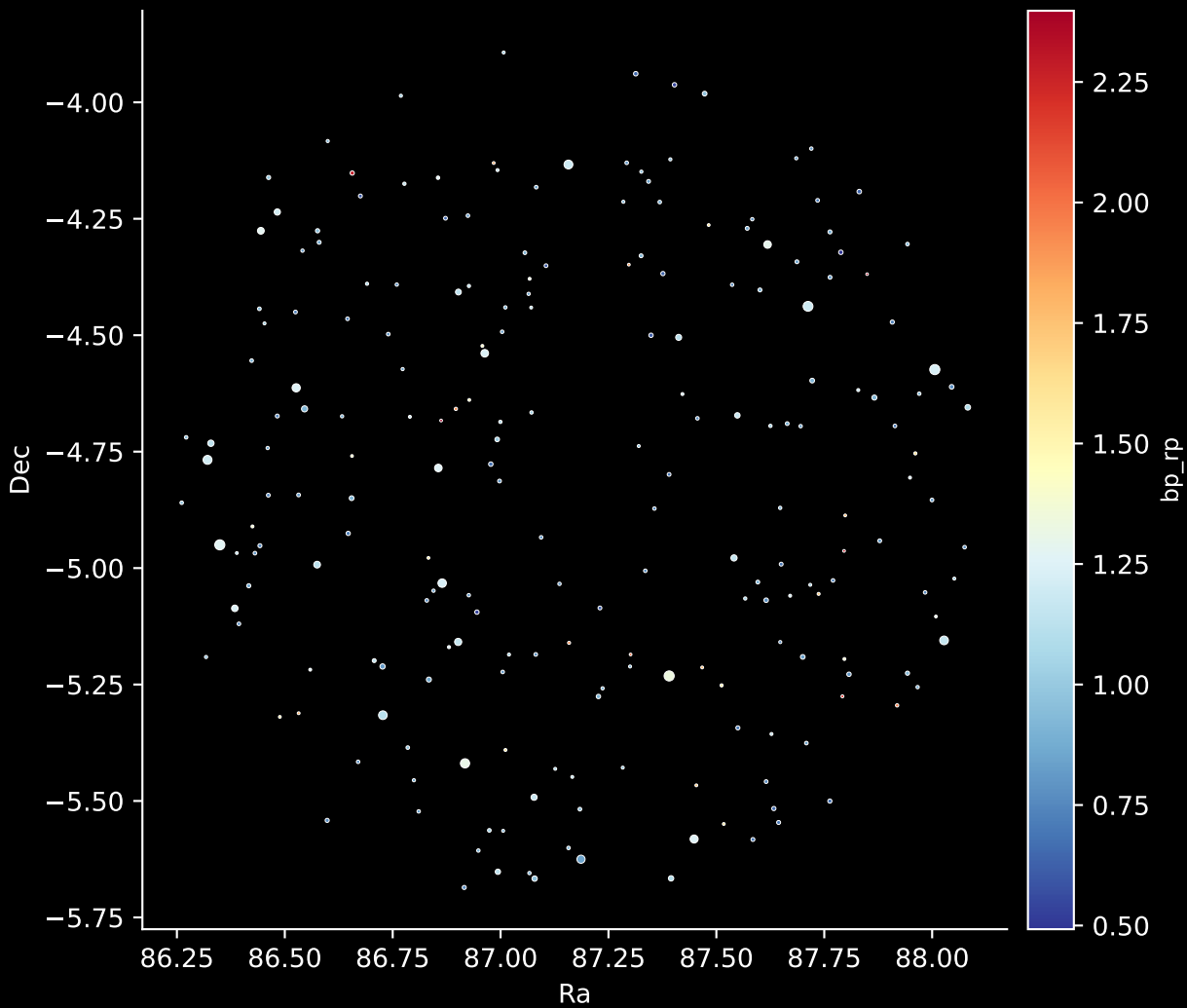
APOGEE DR17 Field: [71-56-O] Stars: 214
