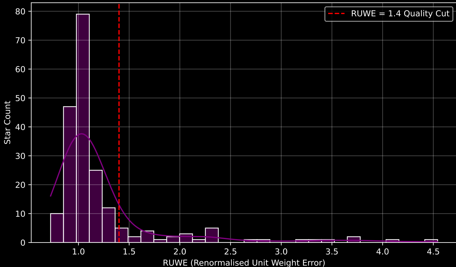
GAPOGEE DR17 Field [71-56-O] RUWE Distribution (n= 205)
