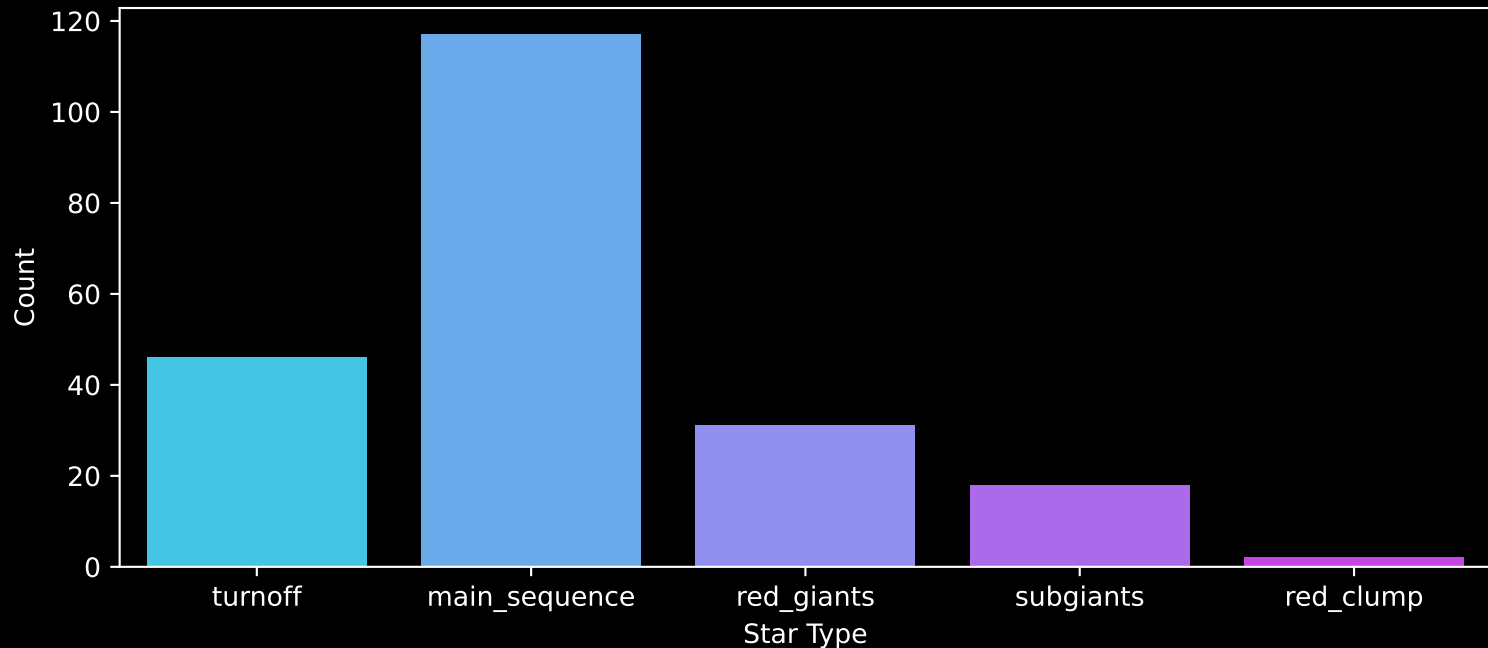
APOGEE DR17 Field: [71-56-O] Count plot of Star Type
