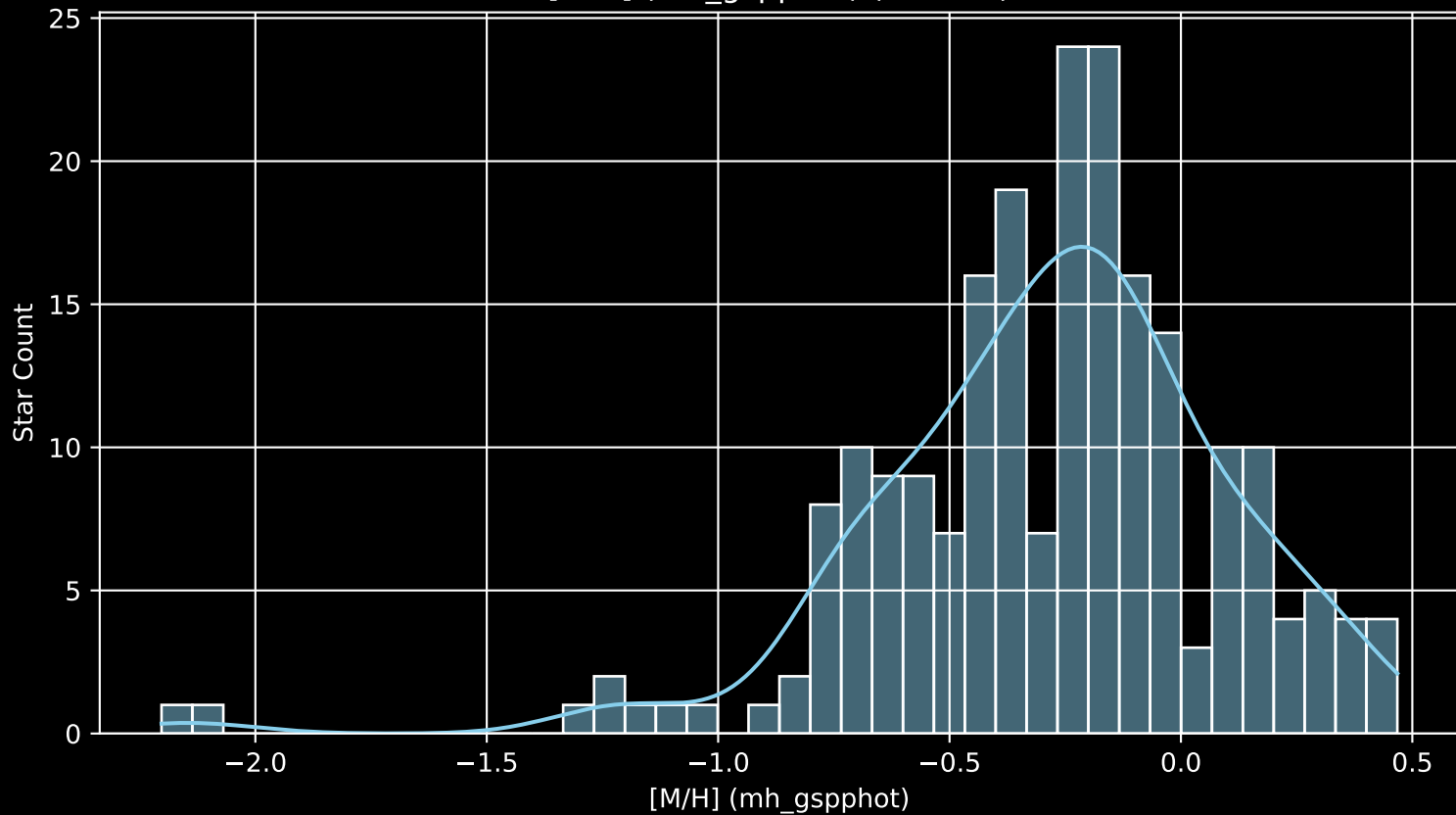
APOGEE DR17 Field: [71-56-O [M/H] (mh_gspphot) (n= 214)
