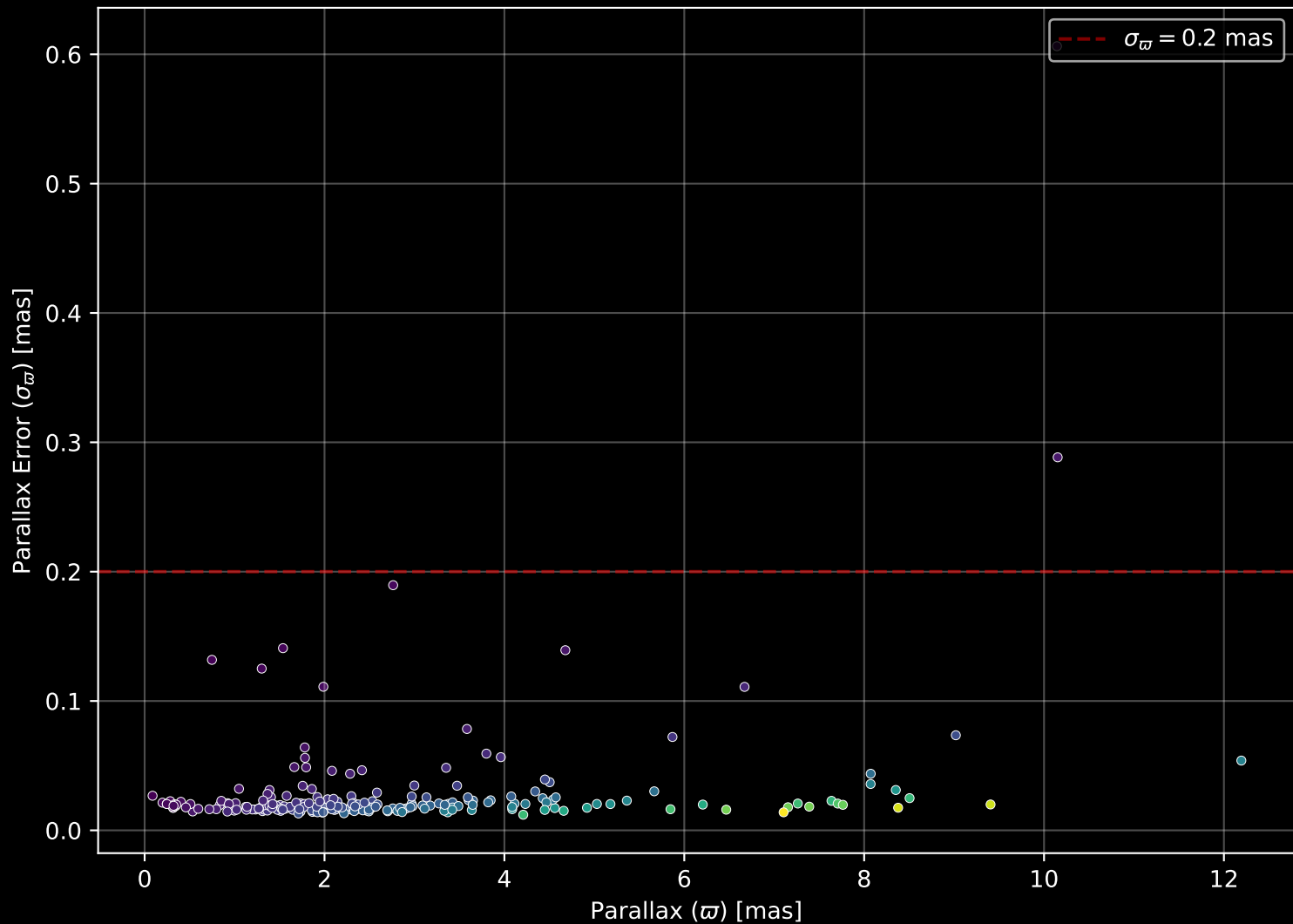
APOGEE DR17 Field: [71-56-O] Parallax Quality (n= 214)
