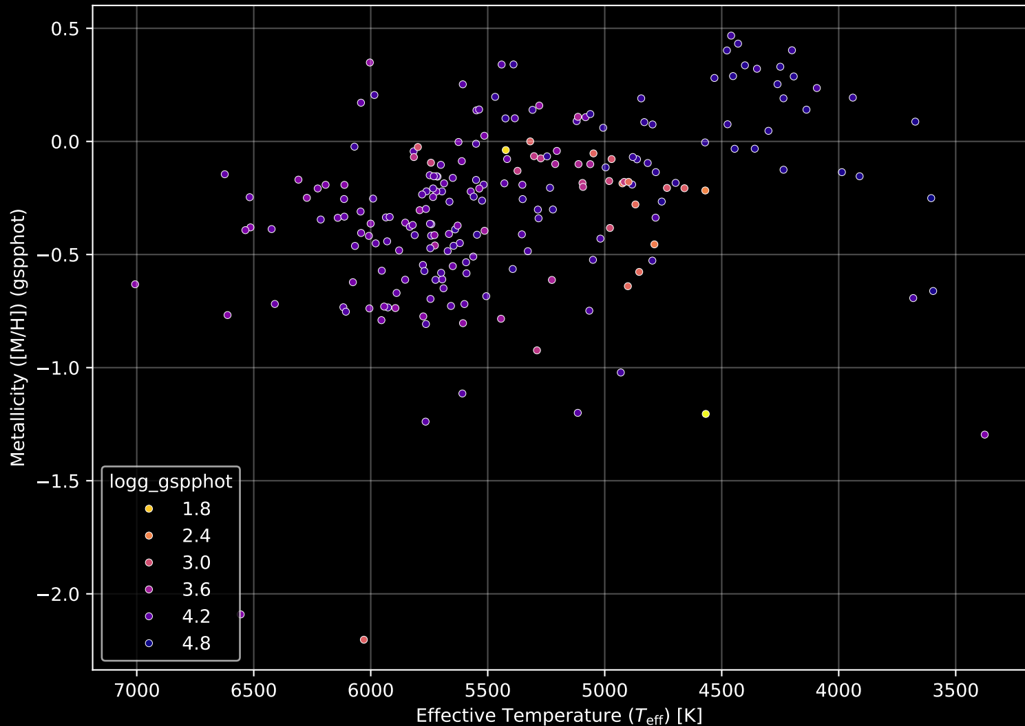
APOGEE DR17 Field: [71-56-O] Stellar Population Parameters (n= 214)
