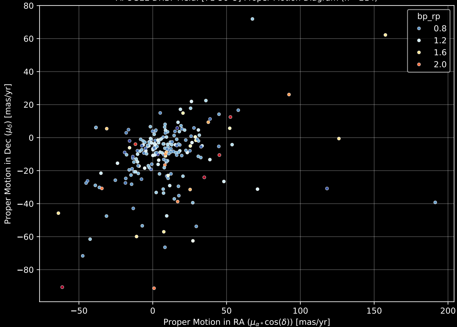
APOGEE DR17 Field: [71-56-O] Proper Motion Diagram (n= 214)
